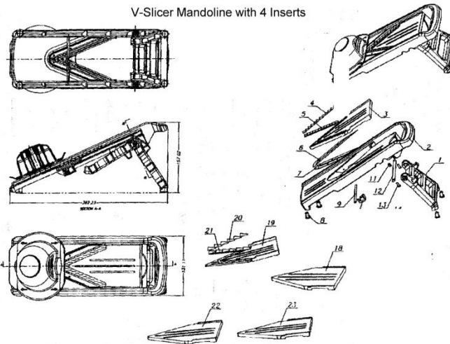
V-Slicer Mandoline with 4 Inserts
